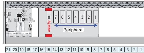
cPCIS-2632R Inside Rear View
