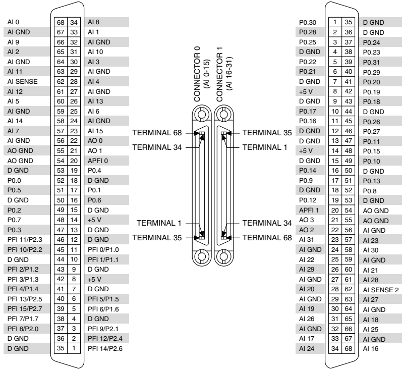
Figure 9. NI PCI/PXI-6289 Pinout
