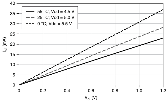
Figure 8. Digital I/O (PFI <0..15>/P1/P2): I_{ol} versus V_{ol}
