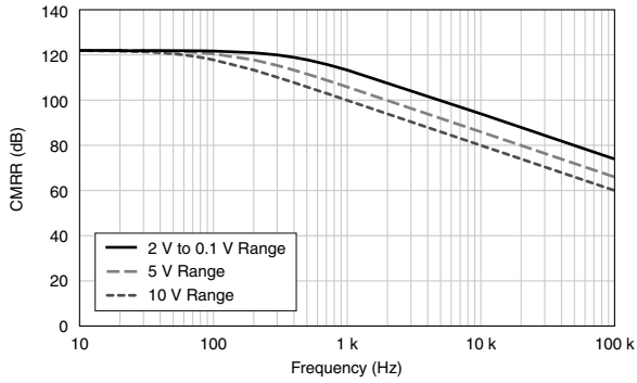
Figure 3. AI CMRR
