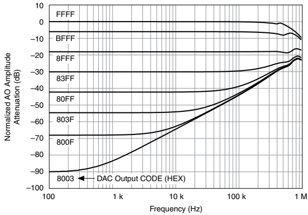
Figure 4. AO External Reference Bandwidth
