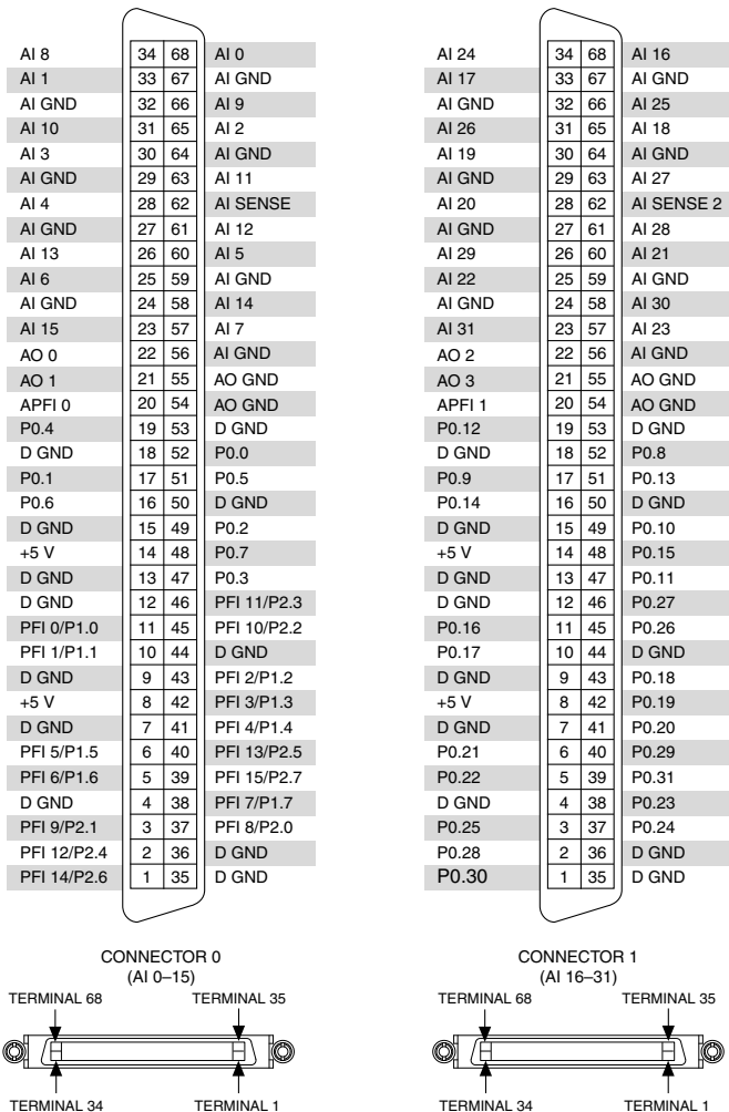
Figure 10. NI USB-6289 Mass Termination Pinout
