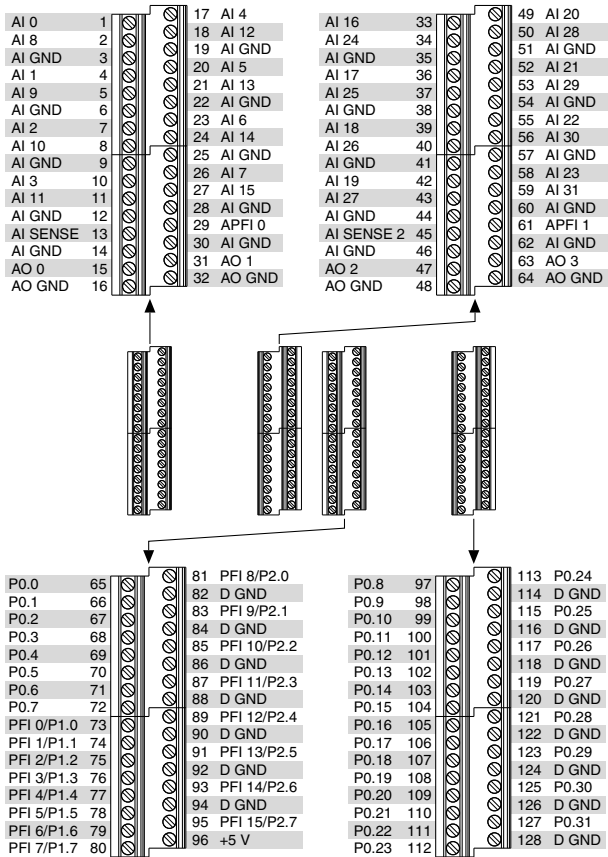
Figure 11. NI USB-6289 Screw Terminal Pinout
