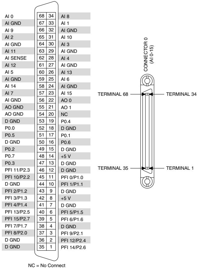
Figure 8. NI PCI/PXI-6221 Pinout
