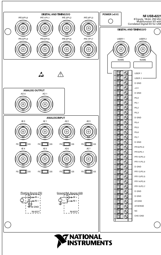
Figure 10. NI USB-6221 BNC Top Panel and Pinout
