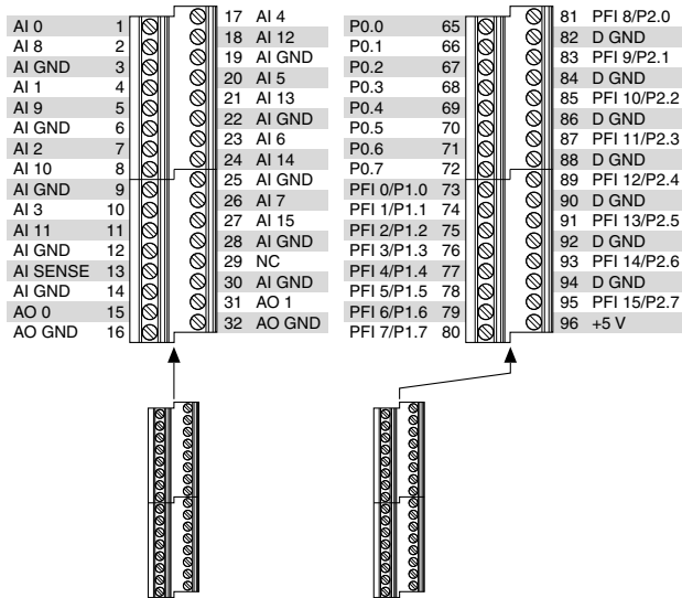
Figure 9. NI USB-6221 Screw Terminal Pinout
