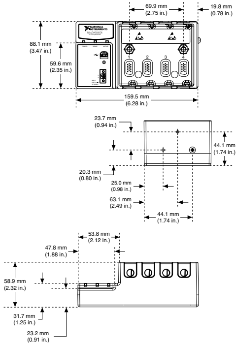
Figure 1. NI cDAQ-9174 Dimensions
