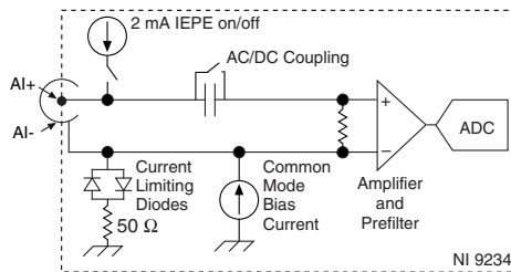
Figure 1. NI 9234 Input Circuitry for One Channel
