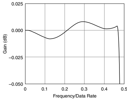
Figure 2. Typical Passband Response for the NI 9234
