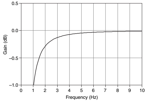
Figure 3. AC Cutoff Frequency Response
