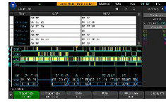
Figure 18: SPI 4wire decode and trigger
