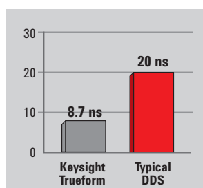
Rise time
