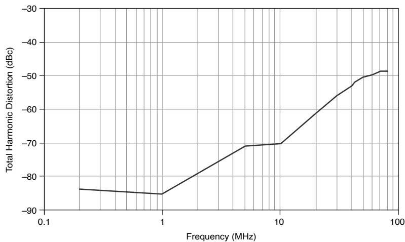
Figure 9. Total Harmonic Distortion, Low-Gain Amplifier Path, Typical
