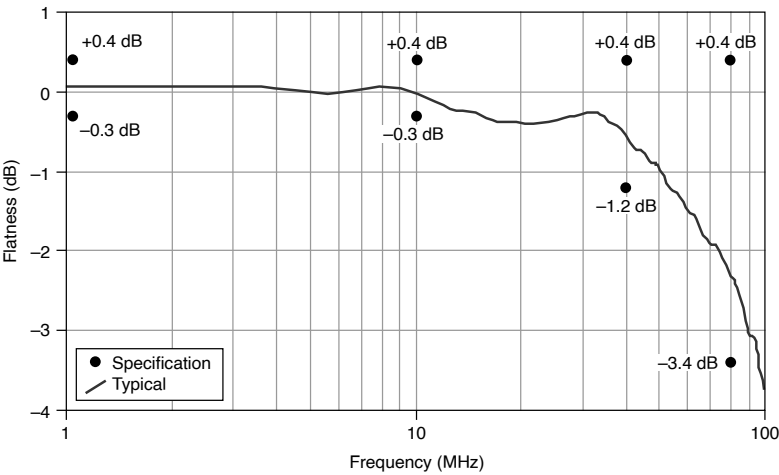
Figure 2. Normalized Passband Flatness, Low-Gain Amplifier Path
