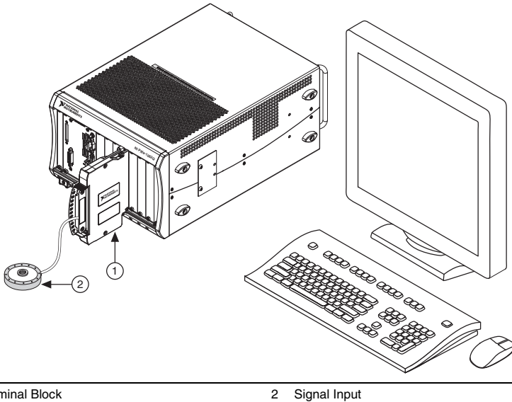
Figure 6. Sample NI PXIe-4304/4305 System
