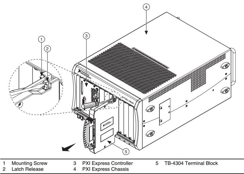
Figure 7. Removing the TB-4304 from the NI PXIe-4304/4305 Module
