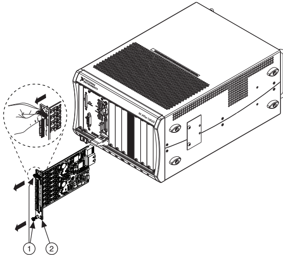
Figure 8. Removing NI PXIe-4304/4305 Modules
