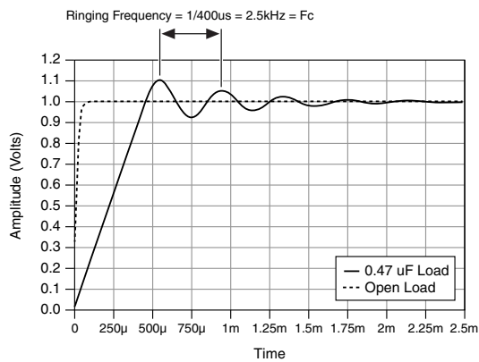
Figure 15. Example of Ringing Frequency
