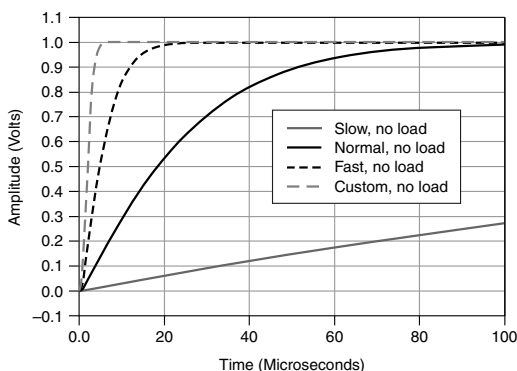
Figure 11. 1 mA Range, No Load Step Response, Nominal
