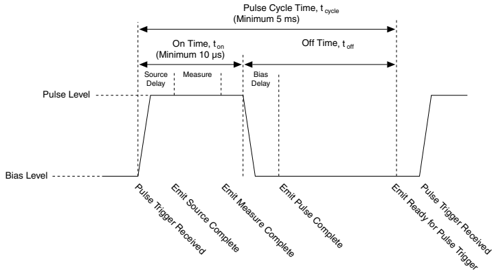
Figure 8. Definition of Pulsing Terminology
