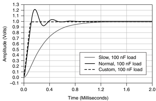
Figure 12. 1 mA Range, 100 nF Load Step Response, Nominal
