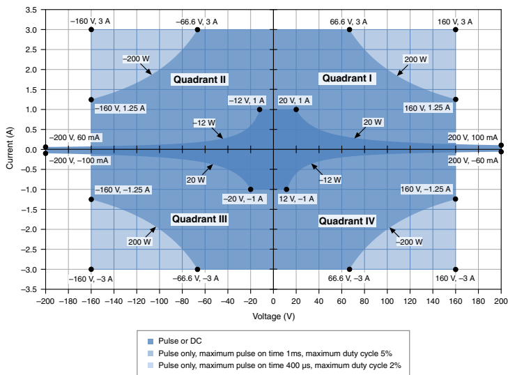
Figure 2. Quadrant Diagram for PXIe-4135 (20W)
