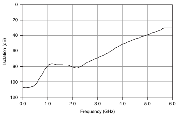
Figure 3. Typical Isolation
