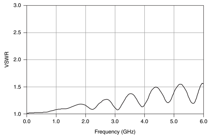
Figure 2. Typical VSWR
