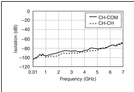
Figure 3. Typical Isolation
