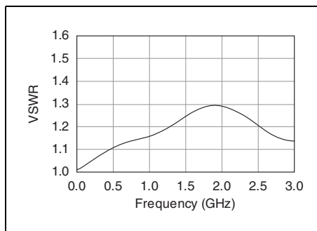
Figure 3. Typical Termination VSWR
