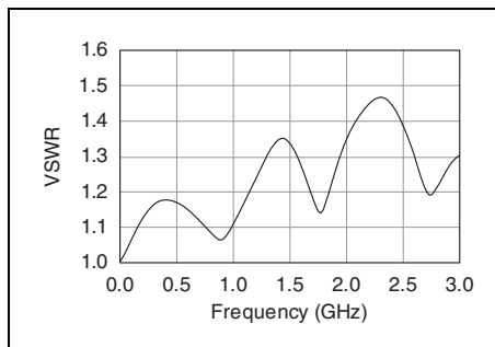
Figure 2. Typical Channel to Common VSWR
