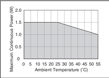
Figure 5. Termination Derating
