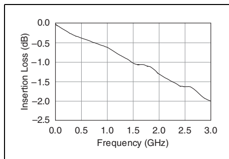
Figure 1. Typical Insertion Loss
