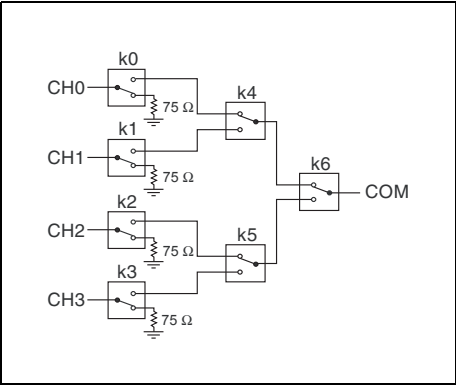
Figure 6. NI PXI-2555 Power-On State
