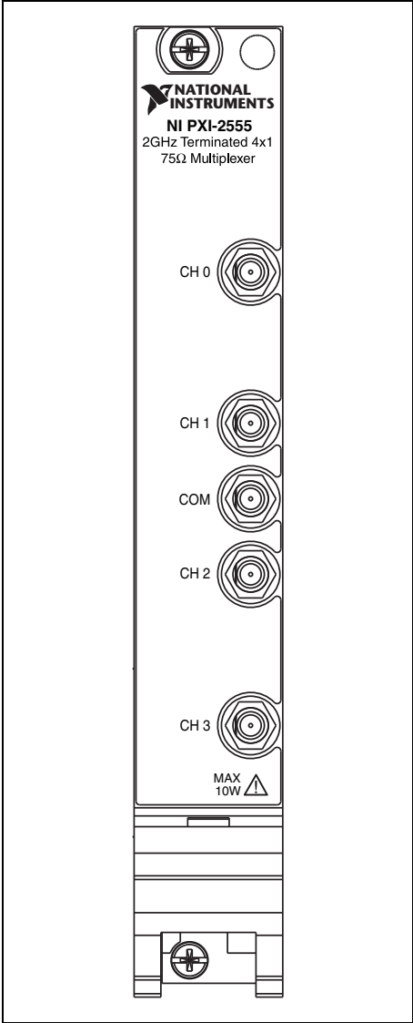
Figure 7. NI PXI-2555 Front Panel Connector
