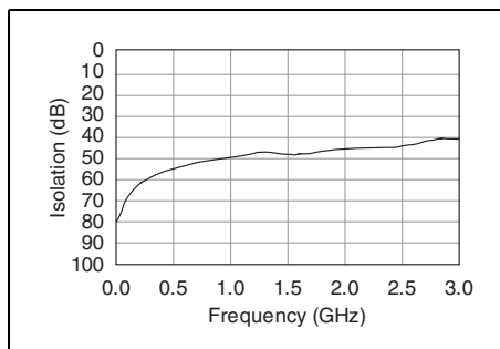
Figure 4. Typical Isolation
