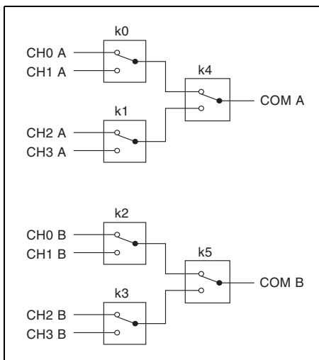
Figure 4. NI PXI-2556 Power-On State
