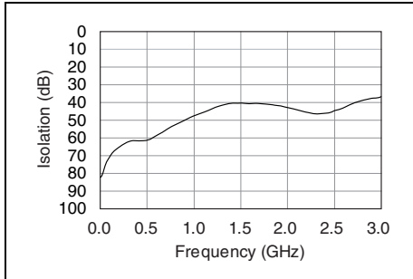
Figure 3. Typical Isolation
