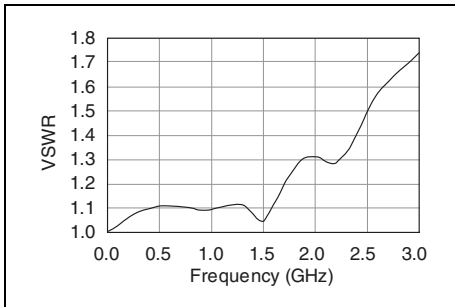
Figure 2. Typical VSWR
