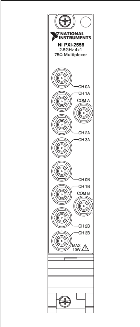
Figure 5. NI PXI-2556 Front Panel Connector
