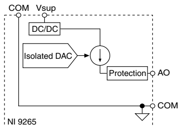
Figure 1. NI 9265 Circuitry
