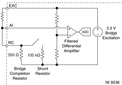
Figure 1. Input Circuitry for One Channel of the NI 9236
