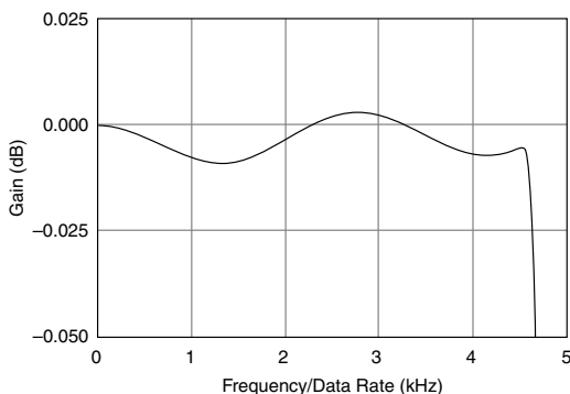
Figure 2. Typical Passband Response for the NI 9236
