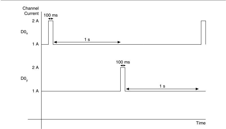
Figure 1. Short-circuit Behavior
