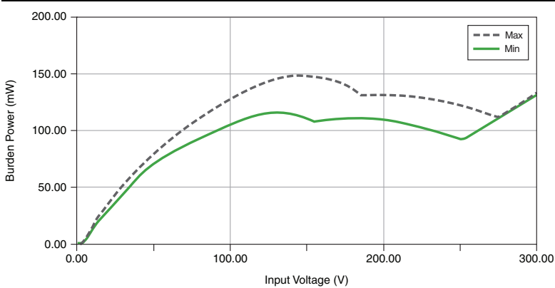
Figure 3. Burden Power Per Channel
