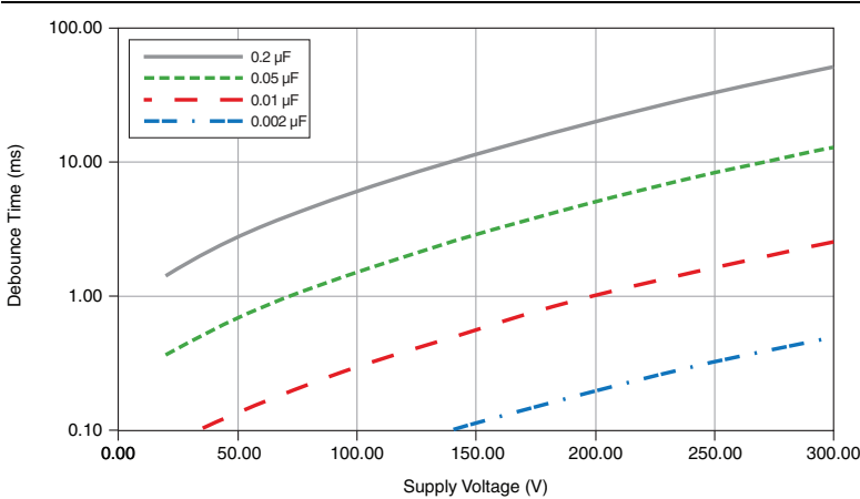
Figure 5. NI 9437 Turn-Off Time
