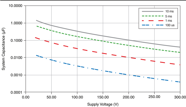
Figure 6. NI 9437 Capacitance Tolerance
