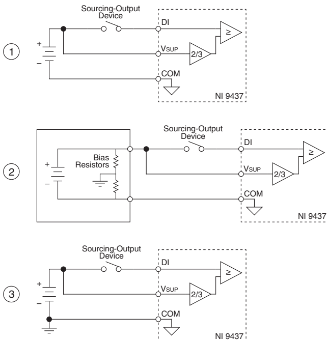
Figure 1. Power Supply Connections to the NI 9437
