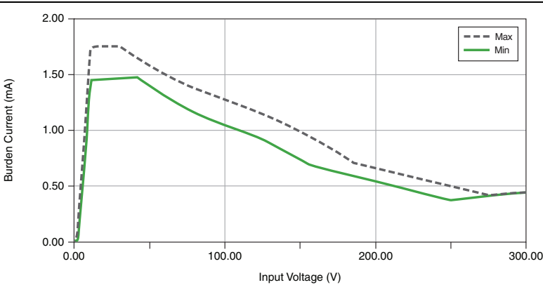
Figure 2. Burden Current Per Channel
