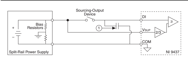
Figure 4. Capacitance Discharge
