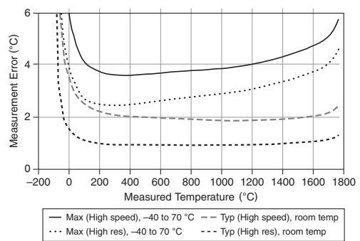
Figure 6. Thermocouple Types R and S Errors
