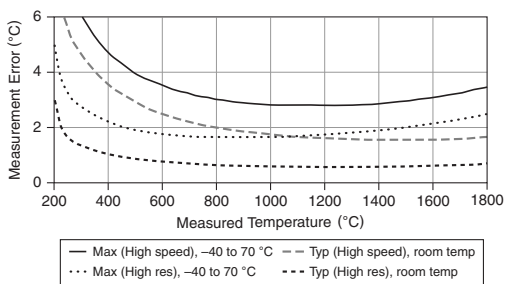
Figure 6. Thermocouple Types R and S Errors
