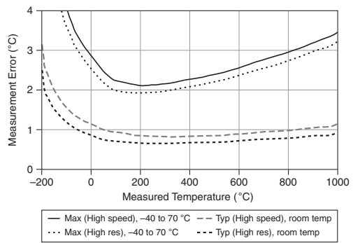
Figure 5. Thermocouple Type B Errors
