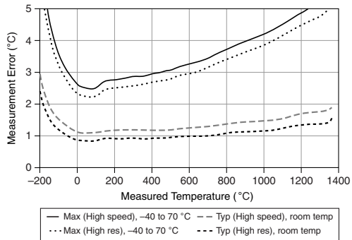
Figure 3. Thermocouple Type K Errors
