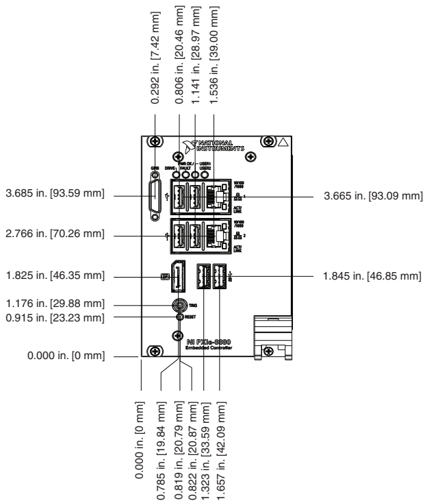
Figure 3-1. NI PXle-8880 Front Panel Layout and Dimensions
