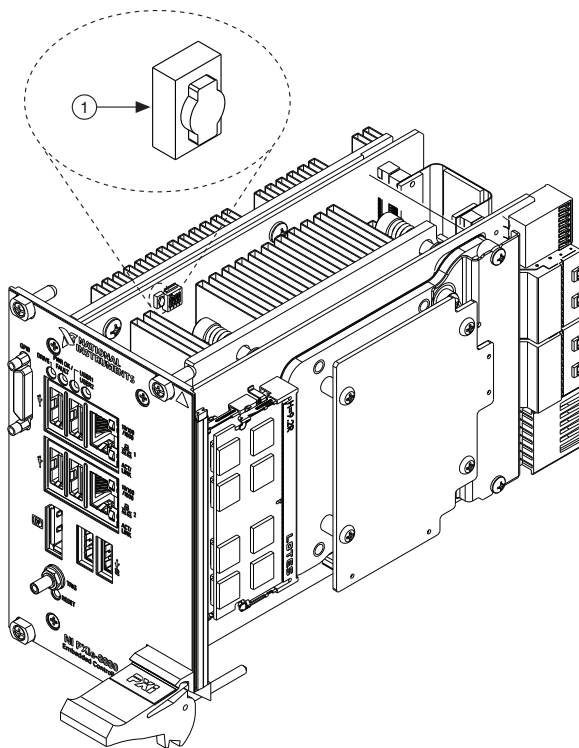
Figure 5-1. Clearing the CMOS Contents
