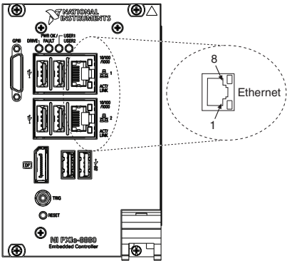
Figure 3-3. Ethernet Connector Location and Pinout
