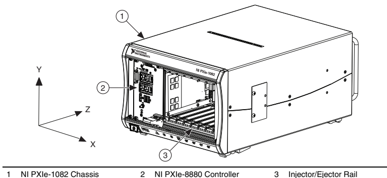
Figure 2-2. NI PXIe-8880 Controller Installed in a PXI Express Chassis
