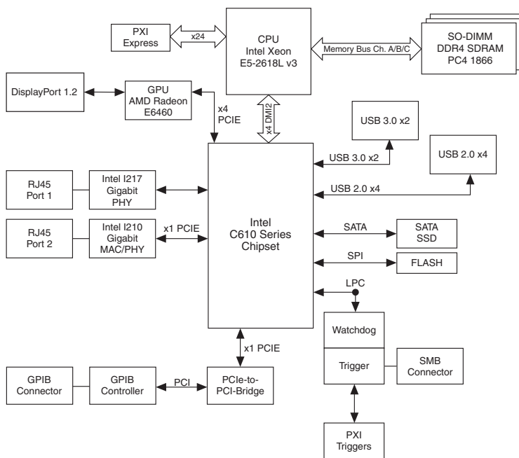
Figure 1-1. NI PXIe-8880 Block Diagram
