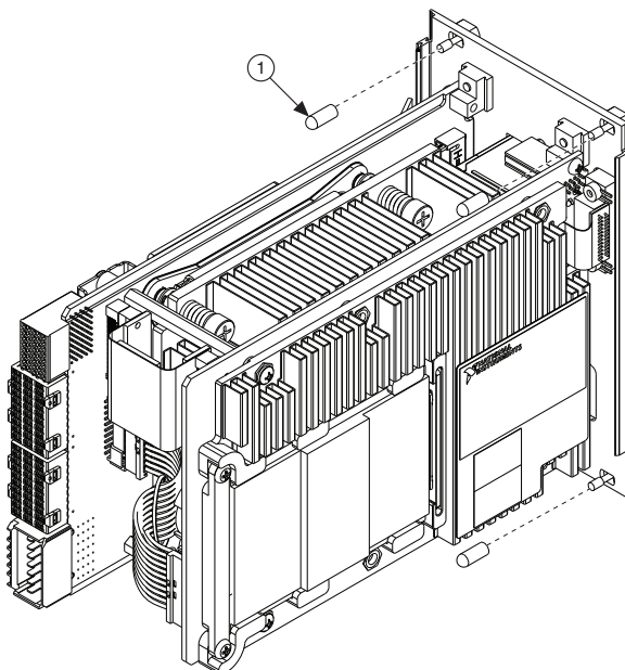
Figure 2-1. Removing Protective Screw Caps
