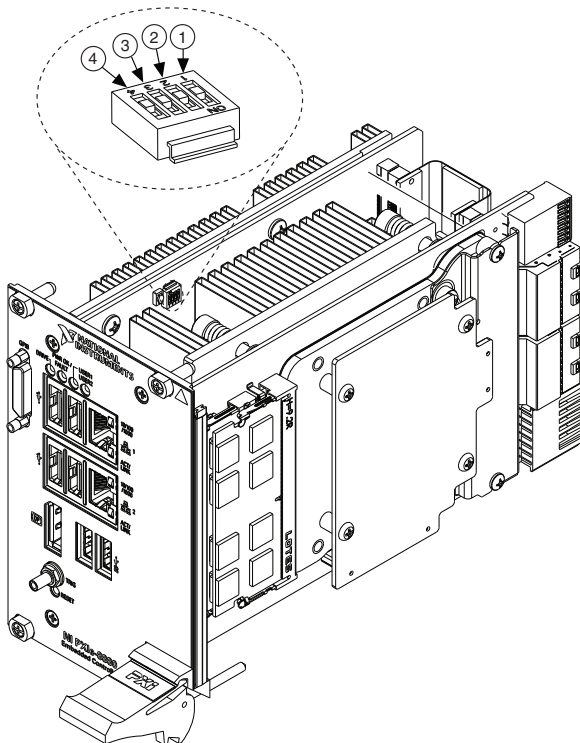
Figure 2-4. LabVIEW RT Configuration Switches
