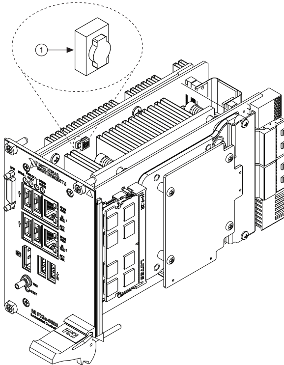
Figure 2-3. Clearing the CMOS Contents
