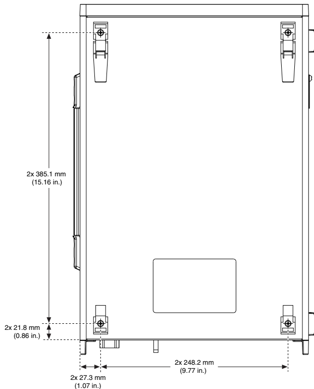
Figure 3. PXIe-1092 Chassis Dimensions (Bottom)
