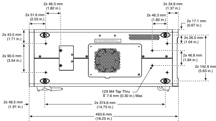
Figure 2. PXIe-1092 Chassis Dimensions (Side)
