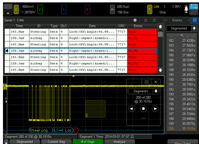
Figure 25. Segmented memory + serial bus decode + zone trigger.
