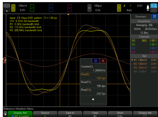
Figure 51. Reference waveforms.
