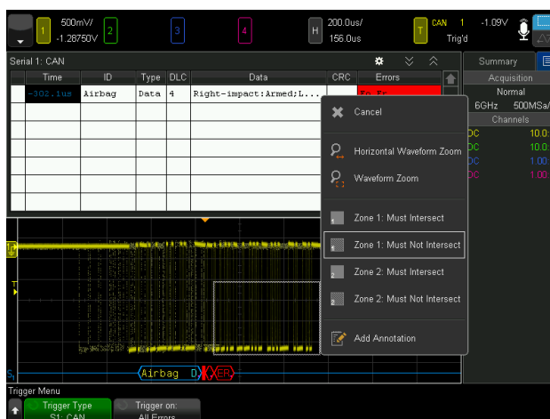
Figure 13. Setting up the zone trigger in addition to a CAN bus error packet trigger.
