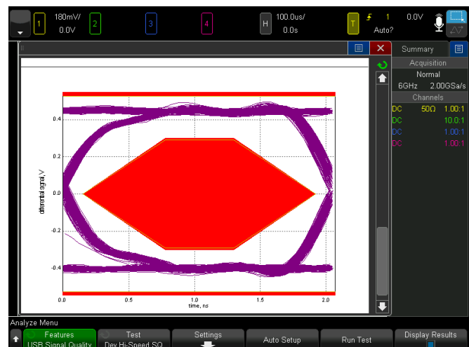
Figure 44. USB 2.0 Hi-speed near-end eye pattern test.
