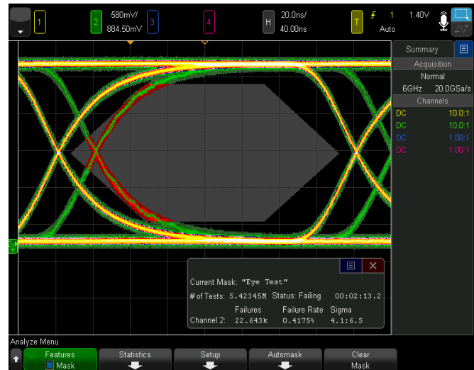
Figure 41. Mask testing of serial data.
