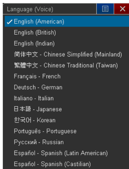
Figure 38. Language list.
