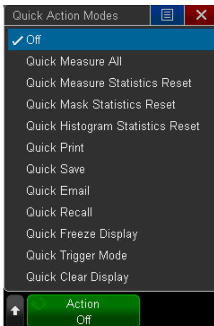
Figure 55. QuickAction menu.
