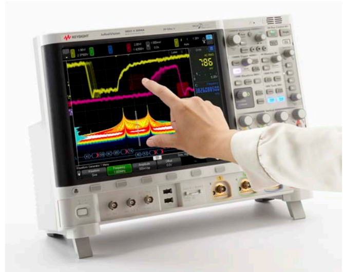
Figure 9. Multi-touch operation.
