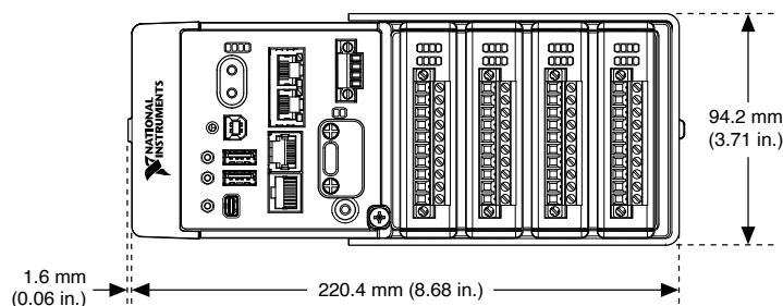
Figure 3. cRIO-9031 Module Immobilization Accessory Dimensions
