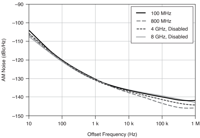
Figure 3. AM Noise for Carrier Frequencies of 100 MHz, 800 MHz, 4 GHz, and 8 GHz (Nominal, Spurs Not Shown)
