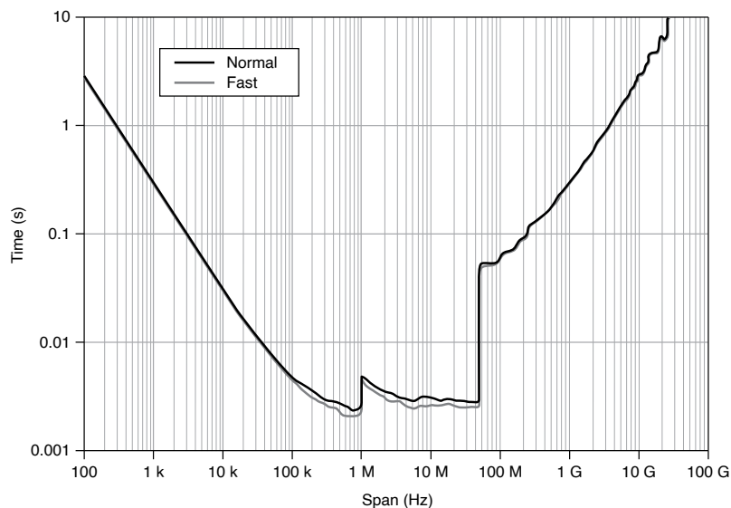
Figure 13. PXle-5668 Analysis Time with 320 MHz and 765 MHz Bandwidth Setting for High Band (Nominal) [24]
