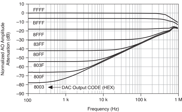
Figure 2. Analog Output External Reference Bandwidth
