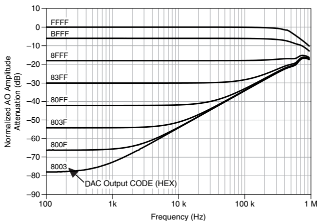
Figure 3. AO External Reference Bandwidth
