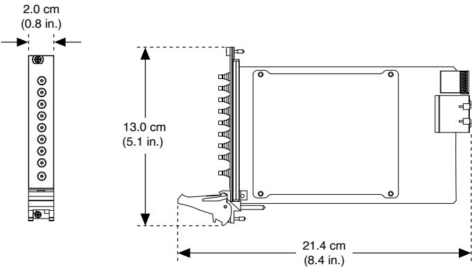
Figure 1. PXle-5105
