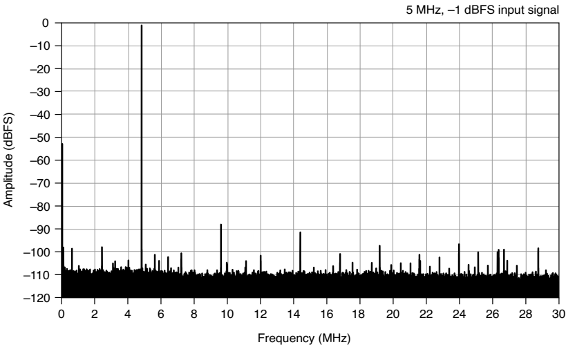
Figure 1. PXIe-5105 Spectral Noise Density, 50 Ω, 0.05 V pk-pk , with Anti-Alias Filter Enabled, Nominal
