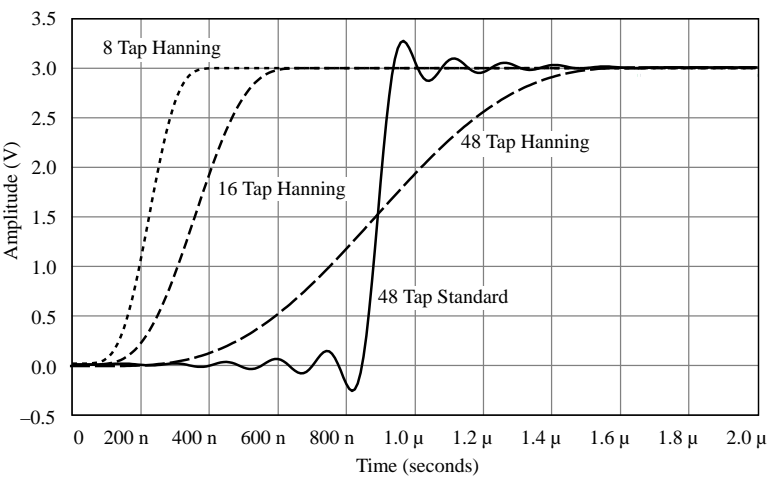
Figure 9. PXI-5922 Frequency Response Using Different Filter Types, Measured
