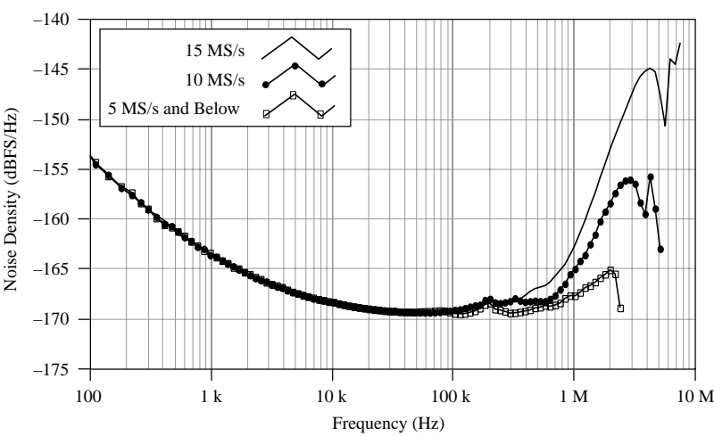
Figure 7. PXI-5922 Noise Density, Measured
