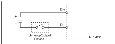
Figure 3. Connecting a Sinking-Output Device to the NI 9422
