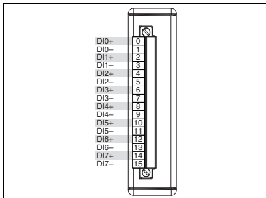
Figure 2. NI 9422 Terminal Assignments
