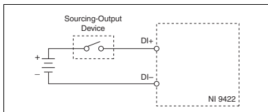
Figure 4. Connecting a Sourcing-Output Device to the NI 9422
