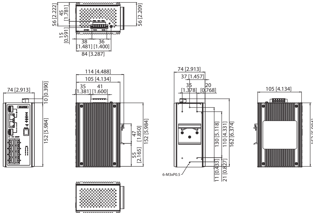
Panel Cut-out Dimensions: 105 (4.137) x 152 (5.984) x 74 (2.91)
