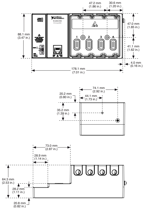
Figure 1. NI cDAQ-9184 Dimensions
