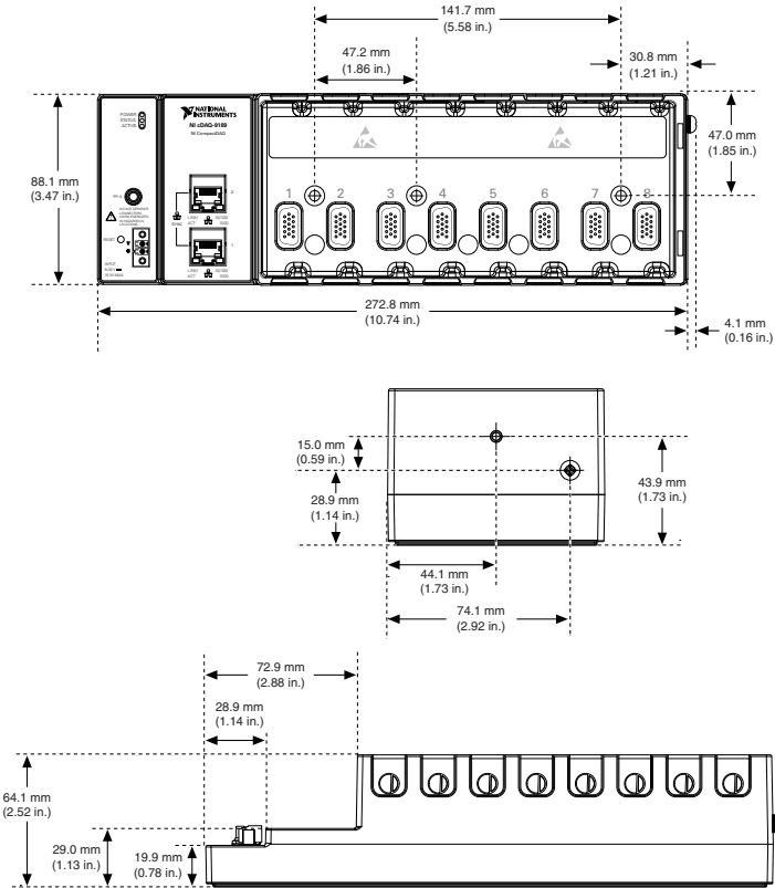
Figure 1. cDAQ-9189 Dimensions
