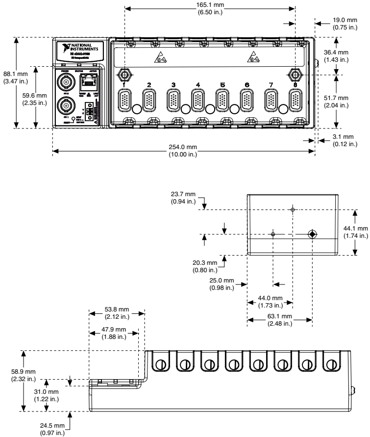
Figure 1. NI cDAQ-9188 Dimensions
