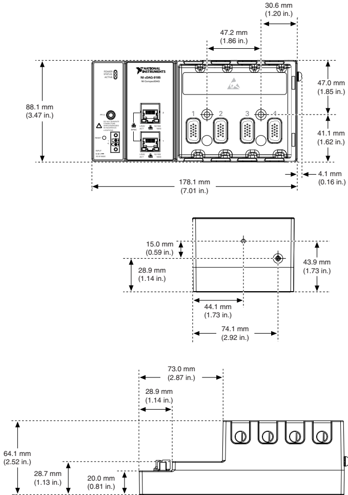
Figure 1. cDAQ-9185 Dimensions
