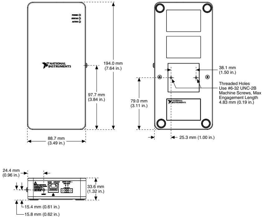
Figure 1. NI cDAQ-9181 Dimensions
