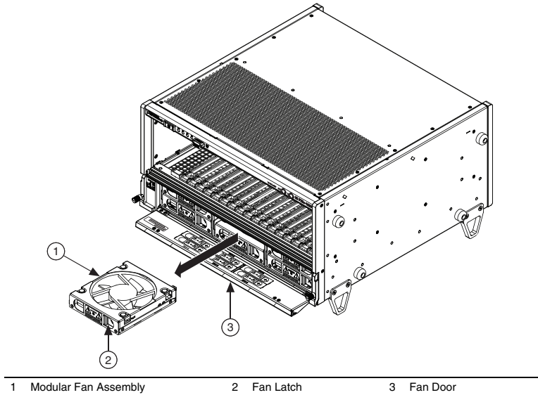
Figure 3-3. PXIe-1086 Chassis with Fan Assembly Removed
