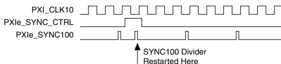
Figure 1-7. PXIe_SYNC100 at 3.33 MHz Using PXIe_SYNC_CTRL as Restart
