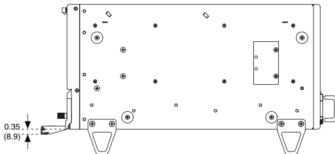
Figure 2-3. Fan Access Door Clearance
