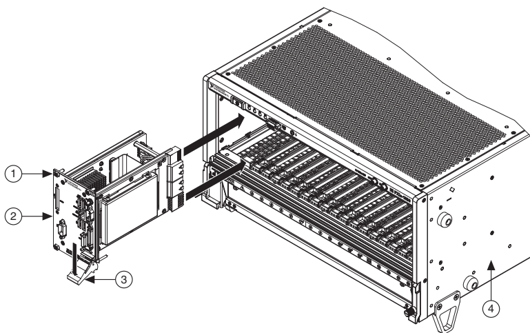
Figure 2-4. Installing a PXI Express System Controller
