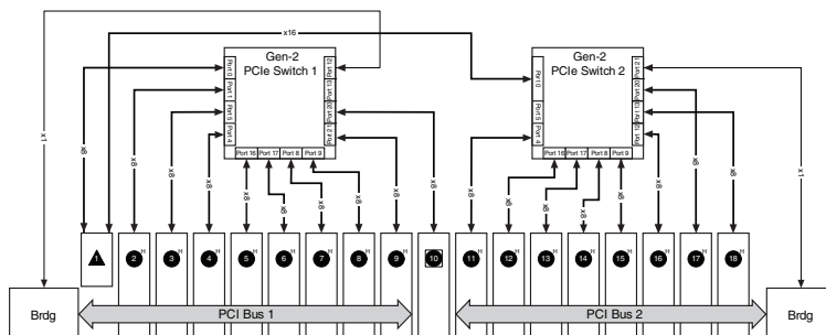
Figure 1-3. PXIe-1086 PCI Express Backplane Diagram
