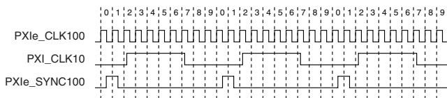
Figure 1-6. System Reference Clock Default Behavior
