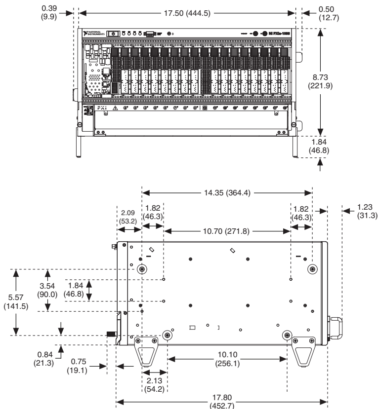
Figure A-1. NI PXIe-1086 Chassis Dimensions (Front and Side)
