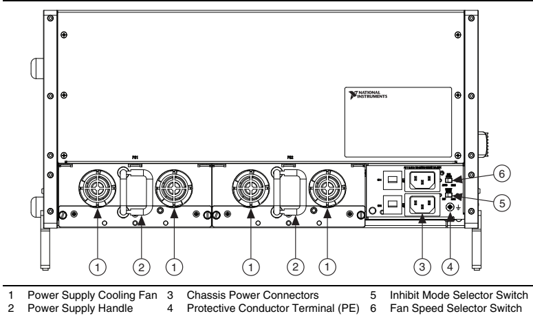
Figure 1-2. Rear View of the PXIe-1086 Chassis
