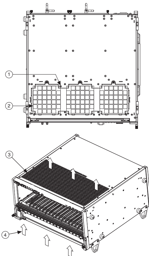
Figure 2-2. PXIe-1086 Vents
