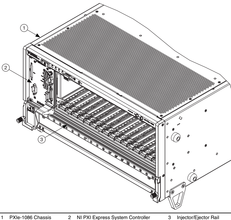
Figure 2-5. NI PXI Express System Controller Installed in an PXIe-1086 Chassis
