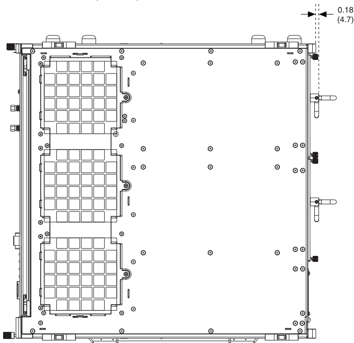
Figure A-2. NI PXIe-1086 Chassis Dimensions (Bottom)
