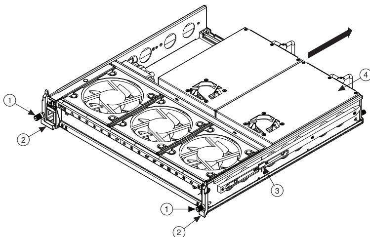
Figure 3-2. PXIe-1086 Power Drawer
