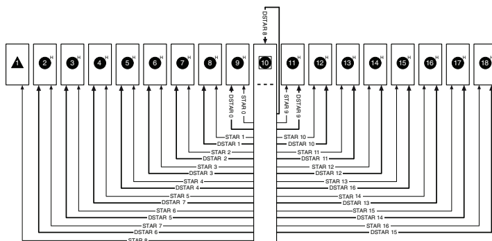
Figure 1-4. PXI Express Star Connectivity Diagram
