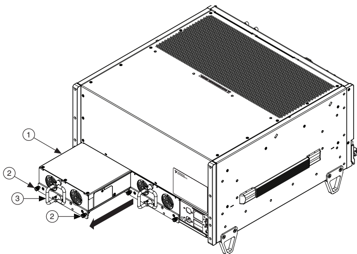
Figure 3-1. Removing Power Supply from PXle-1086 Chassis
