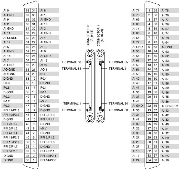
Figure 8. NI PCI/PXI-6225 Pinout
