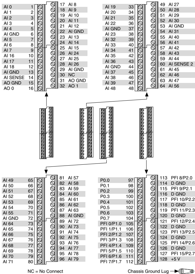
Figure 9. NI USB-6225 Screw Terminal Pinout
