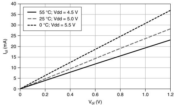
Figure 7. DIO PFI/Port 1/Port 2: I_{ol} versus V_{ol}
