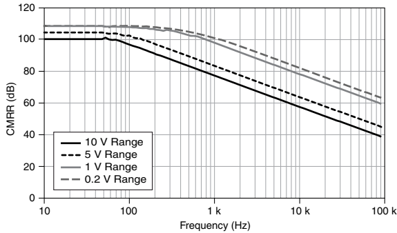
Figure 3. AI CMRR
