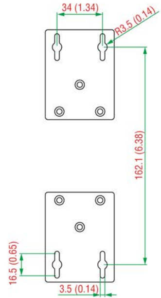
Panel-Mounting Kit
