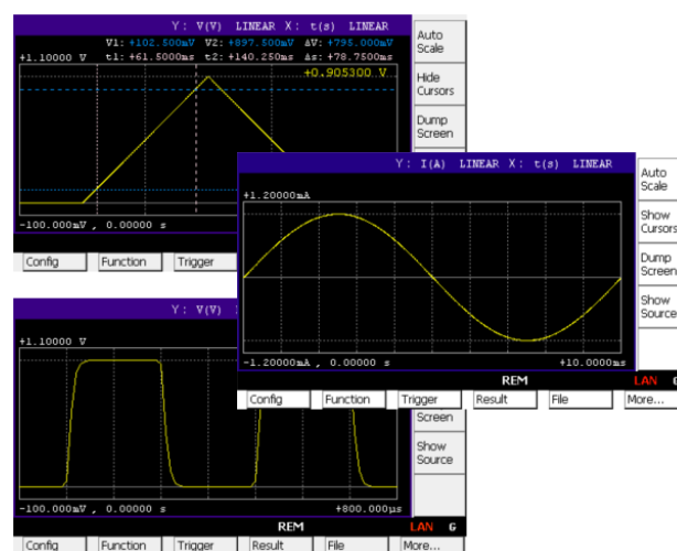
Figure 9. Graph View allows you to view output waveform in the time domain
