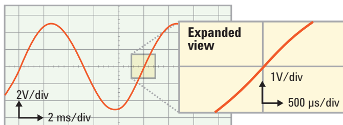
Figure 11B. Sinusoid waveform comparison at 100 Hz (B2961A/B2962A)
