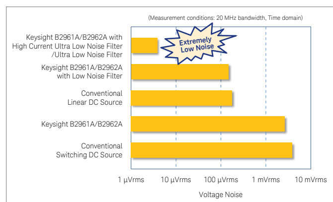
Figure 5. HC-ULNF and ULNF dramatically reduce output noise
