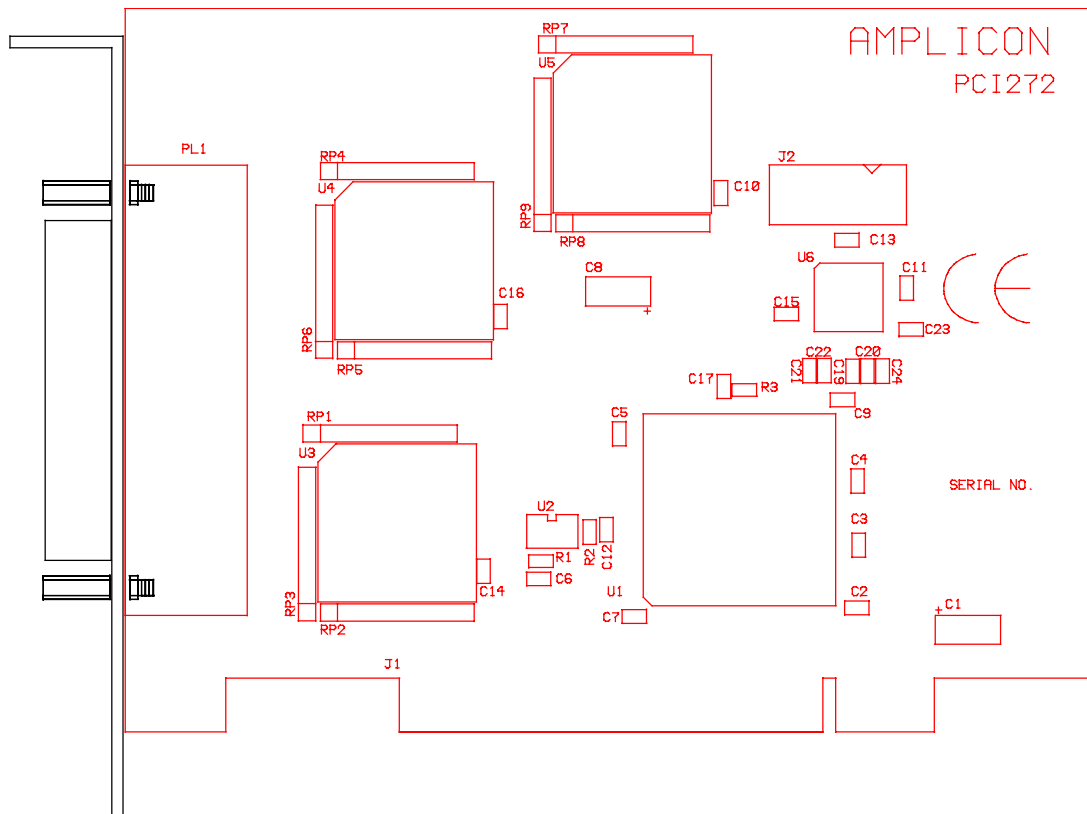
FIGURE B.1 PRINTED CIRCUIT LAYOUT
