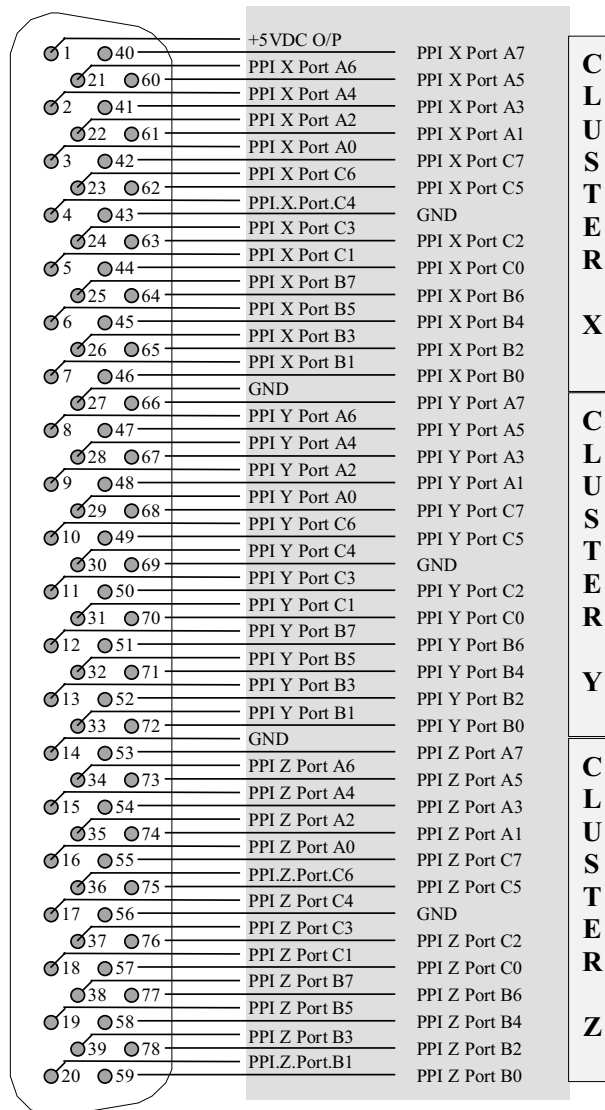
FIGURE 3.1 78 WAY D-TYPE CONNECTOR (SK1 - USER I/O)
