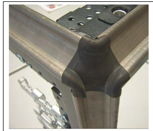
Figure 7: Conductive Textile Gasket
