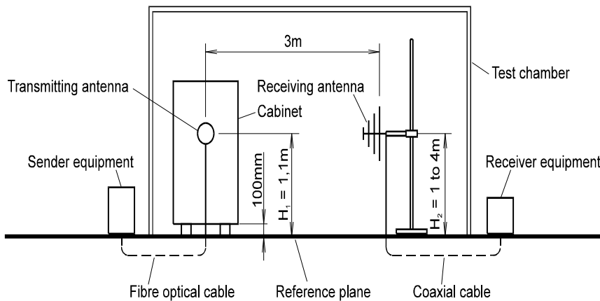
Figure 5: Set-up for measurement of the shielding
