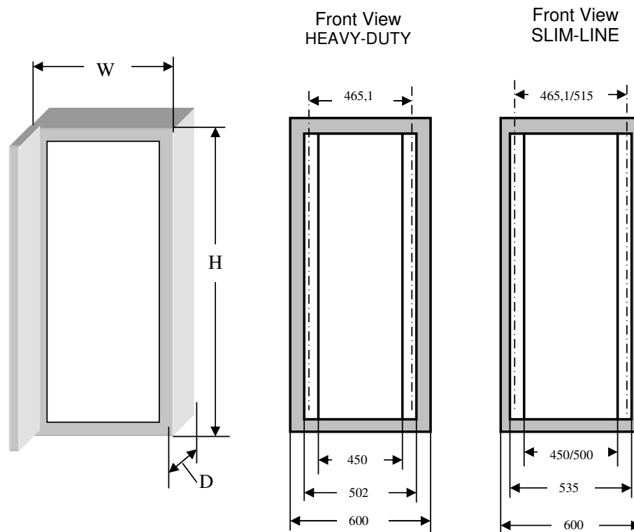
Figure 1: Assembly dimensions for HEAVY-DUTY and SLIM-LINE
