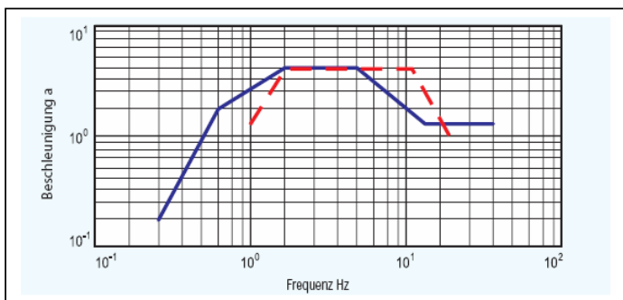
Figure 9: Seismic test according to IEC 61587-2
