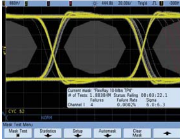
Mask testing uncovers an infrequent signal anomaly.
