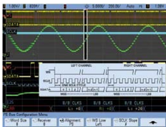
On-screen serial decode of an SPI packet
