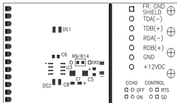
Figure 1. R9 Resistor & Baud Rate
