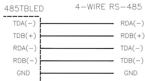
Figure 2. 4-Wire RS-485
