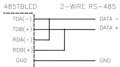
Figure 3. 2-Wire RS-485
