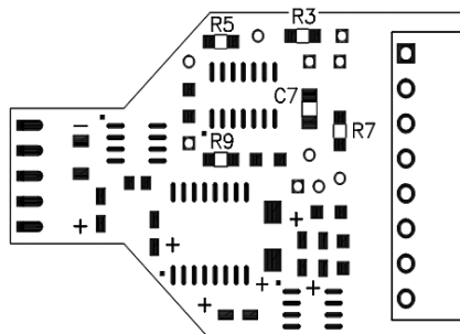
Figure 1. PC Board Layout - Top
