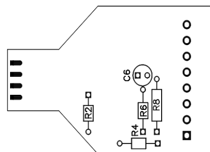
Figure 1. PC Board Layout - Bottom
