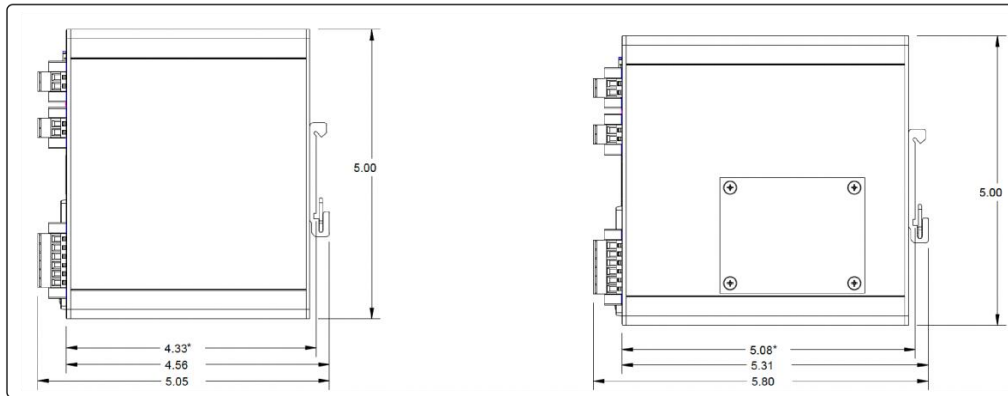
Figure 3. Cisco Catalyst IE3100 side view dimensions
