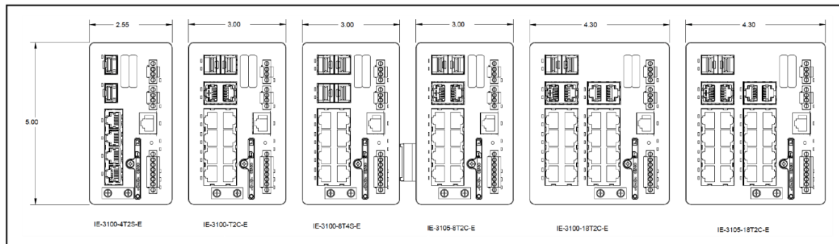
Figure 4. Cisco Catalyst IE3100 front view dimensions
