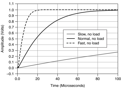
Figure 3. 1 mA Range, No Load Step Response, Nominal
