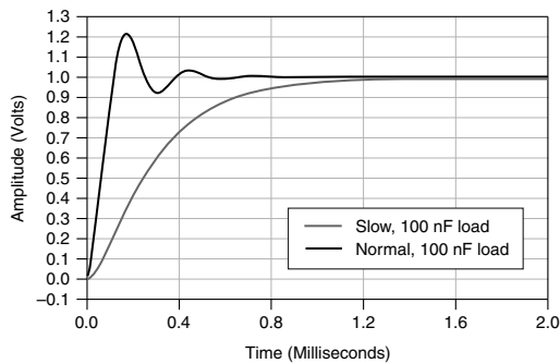
Figure 4. 1 mA Range, 100 nF Load Step Response, Nominal
